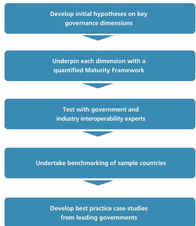
Figure 2: Research methodology
